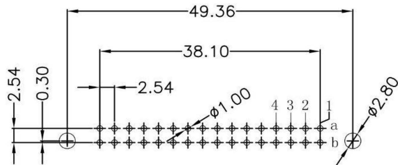
PCB LAYOUT(RECOMMENDED) (TOP VIEW TOL. :±0.05)
